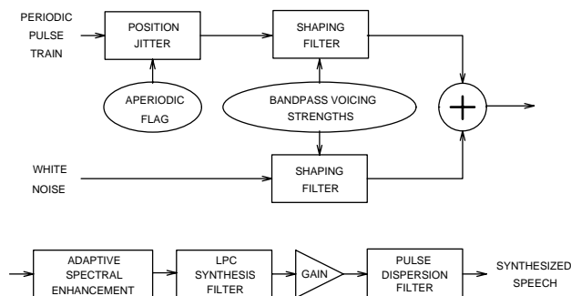
Figure 1: MELP synthesizer.
