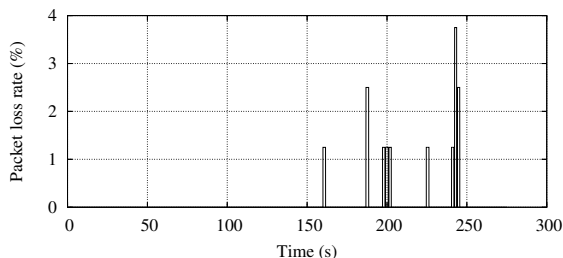
Figure 5: Packet loss rate as a function of time for the VTSS technique.
